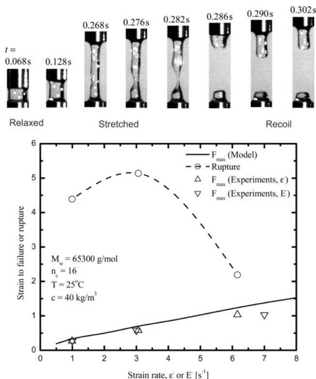
Figure 13. (a, top) Images showing rupture of 2.4 wt % HEUR22-2. The applied strain rate is \dot{\epsilon} = 3 \text{ s}^{-1} . (b, bottom) Strain to failure and strain to rupture during the extension of 4 wt % HEUR22-2 filament.
