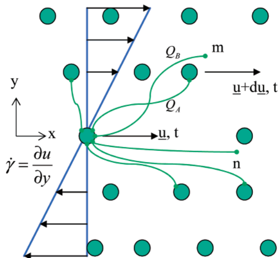
Figure 2. Schematic of two hydrophobic ends “m” and “n” in a lattice of micelles undergoing shear. The “m” end is likely to experience more interactions with neighboring micelles compared to the “n” end due to the differential velocity.
